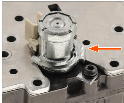
Factory bracket commonly broken
