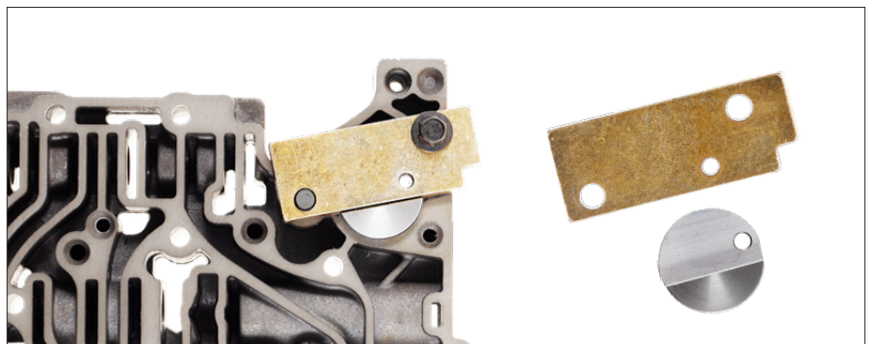
Factory bracket commonly broken
