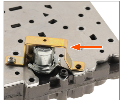
TransGo HD retaining bracket
